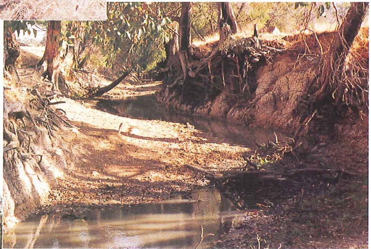
C3 foreshore on the Sabina River. Soil is being washed away from between tree roots and the undermined trees are at risk of falling into the river. This will cause ongoing erosion problems.
