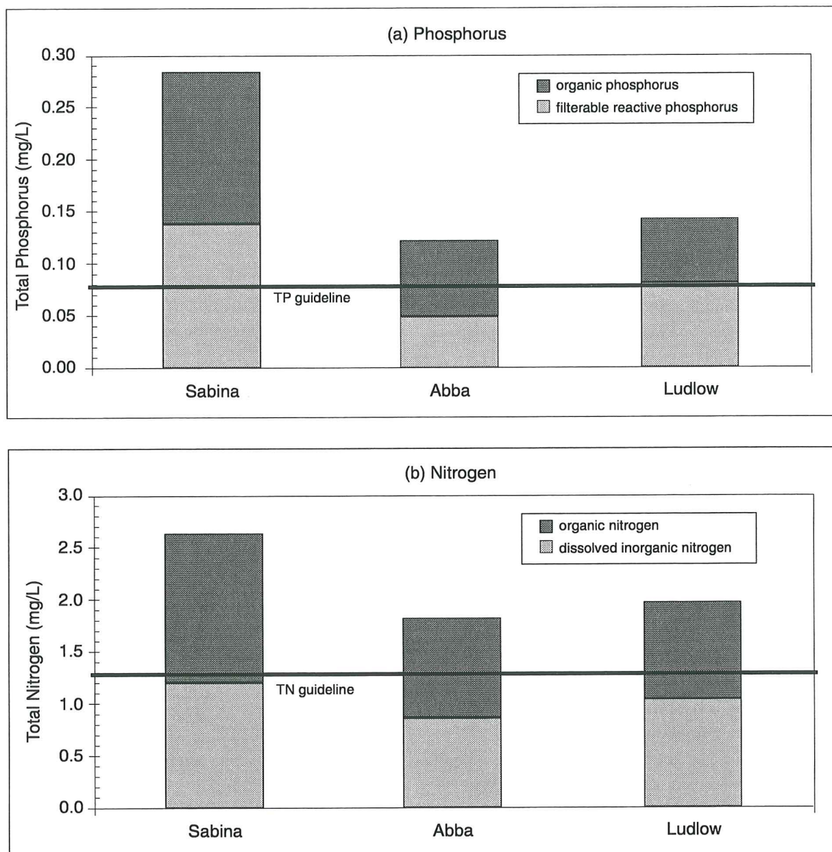
Figure 5: Forms of nutrients in the Sabina, Abba and Ludlow Rivers: (a) total phosphorus; (b) total nitrogen
