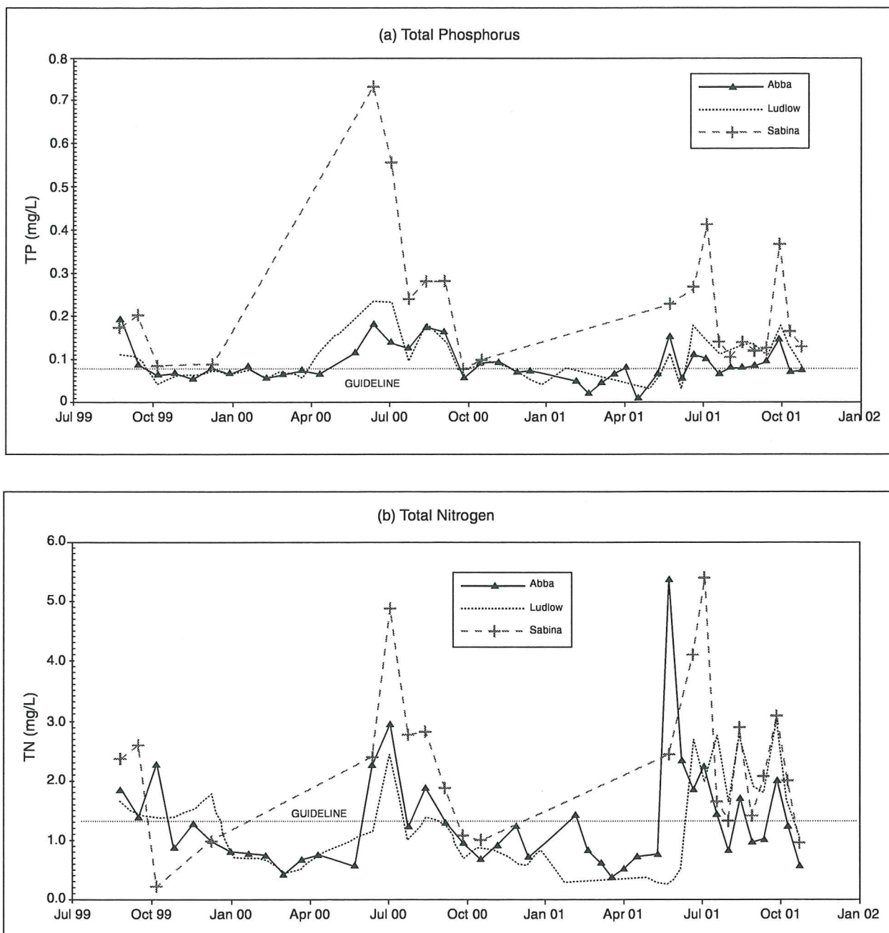
Figure 4: Total nutrient data for the Sabina, Abba and Ludlow Rivers: (a) total phosphorus; (b) total nitrogen
